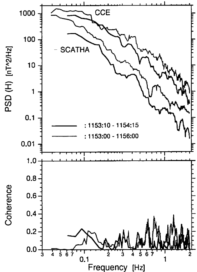
Figure 6a. The coherence between the AMPTE/CCE and SCATHA measurements for the H magnetic component for the intervals of 1153:10 to 1154:15 UT (solid lines) and 1153:00 to 1156:00 UT (dotted lines). (Top) The power spectrum density and (bottom) coherence are plotted. The numbers of the degree of freedom for the spectral estimate, which is twice the N band, are 30 and 18 for the long and short intervals, respectively.
