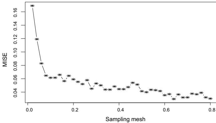
Fig. 8 \text{MISE}(\delta) for the first derivative of the regression function with n = 105
