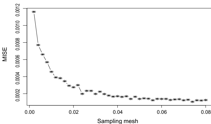
Fig. 6 \text{MISE}(\delta) for bidimensional OU processes with n = 105
