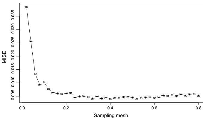
Fig. 2 \text{MISE}(\delta) for a one-dimensional OU process where n = 105
