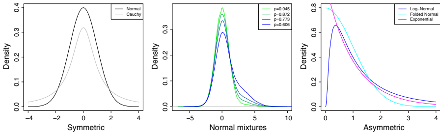
Fig. 1 The left figure shows the symmetric Normal and Cauchy density curves. The middle figure shows the density curves of Normal mixtures of the form pN(0, 1) + (1 - p)N(2, 2) , for 0 < p < 1 . The rightmost figure shows the three ‘highly’ asymmetric densities which, in order of increasing asymmetry, are Log-Normal, Folded Normal and Exponential
