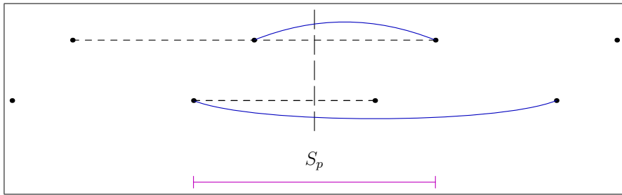
Fig. 1 A co-jump and intervals that determine the covariance structure
