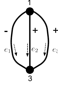
Figure F.2: The graph \hat{G} .
