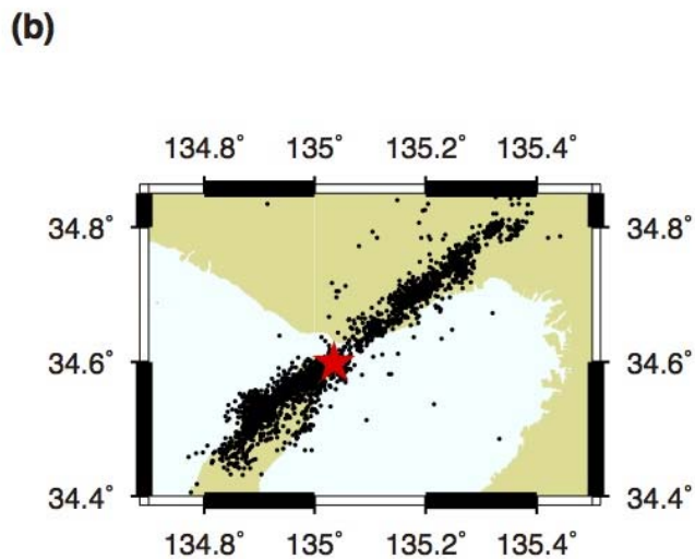
1995 Hyogo-Ken-Nanbu earthquake (M7.3)
