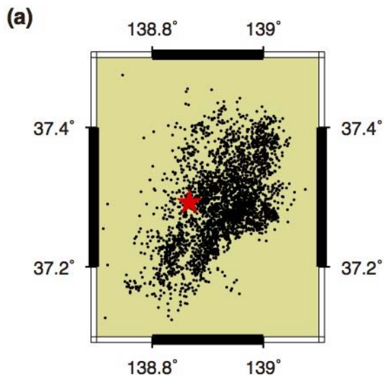
2004 Chuetsu earthquake (M6.8)
