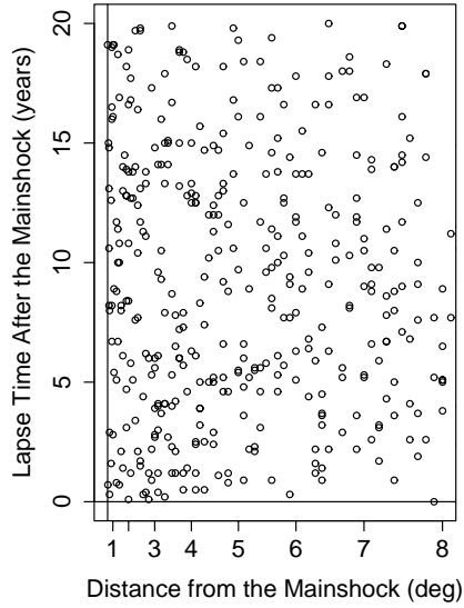
(a) No change-point
