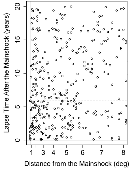
(b) Relative quiescence
