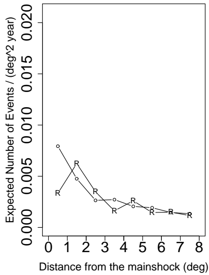
(b) next 14 years span
