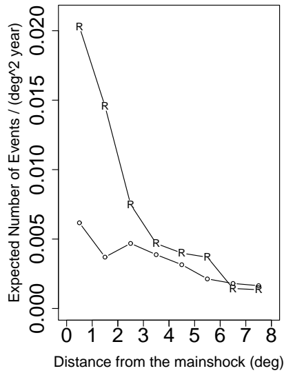
(a) first 6 years span
