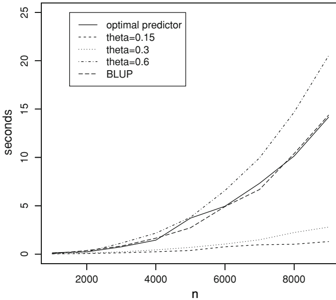
Fig. 1 The time required for the calculation of each predictor for various taper ranges
