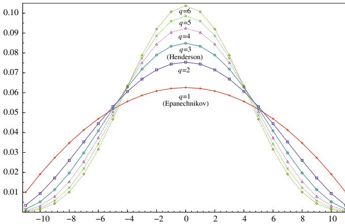
Fig. 2 Plot of the normalised kernel weights associated with the covariance matrix of the non-invertible MA( q ) process \varepsilon_t = (1 - B)^q \xi_t , for q = 1, \dots, 6 and h = 10
