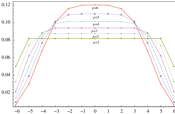
Fig. 1 Plot of the kernel weights associated with the covariance matrix of the AR( p ) process (1 + 0.64B)^p \varepsilon_t = \xi_t , for p = 1, \dots, 6 and h = 6
